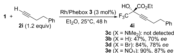
Scheme 1. Electronic tuning of Rh/Phebox complex 3 .
